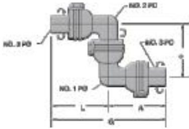
Style No. 10 (Three Planes of Rotation)
